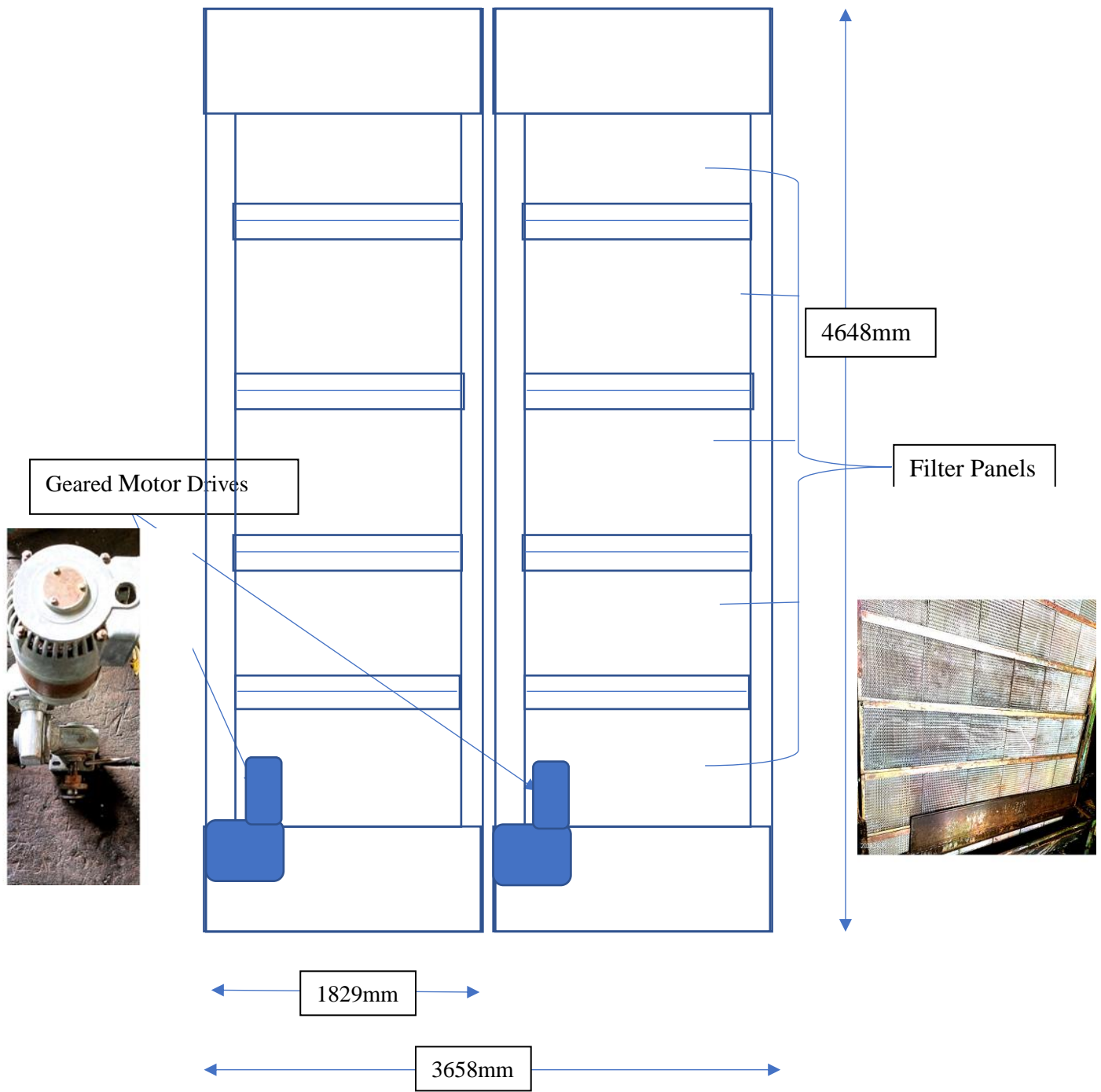
Figure 2: Filter Panel Drive system
